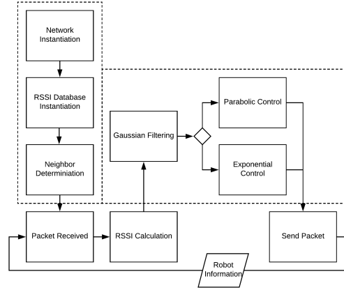
Fig. 3: Algorithm Overview
