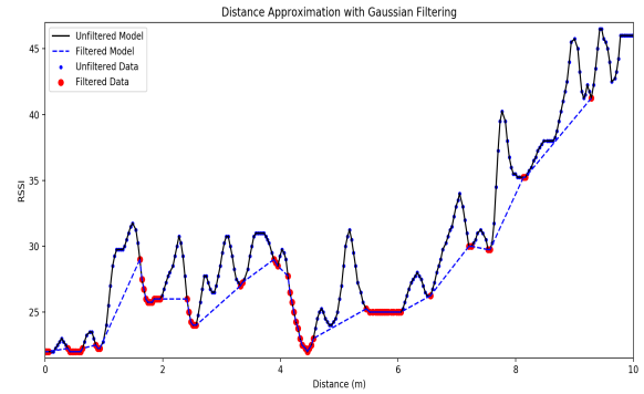
Fig. 5: Gaussian Filtering of Observed RSSI Measurements
