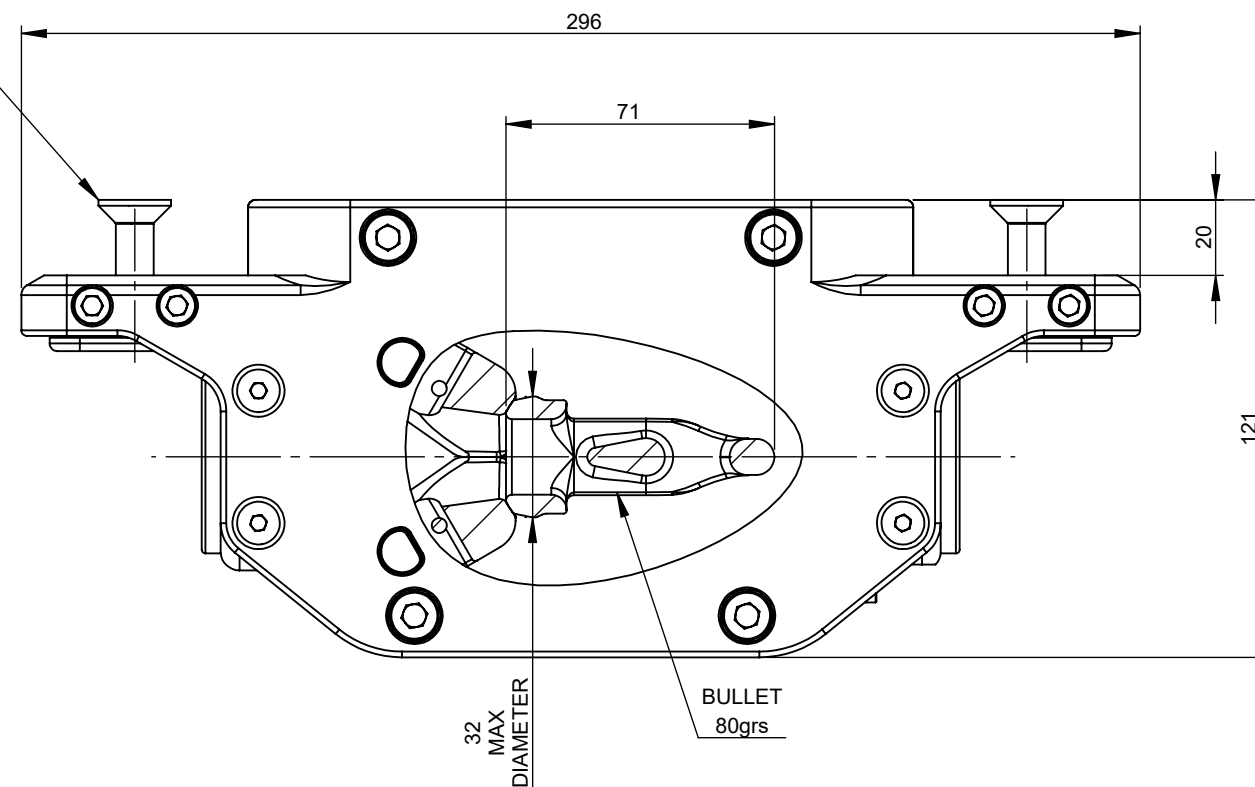
LOCKED POSITION
