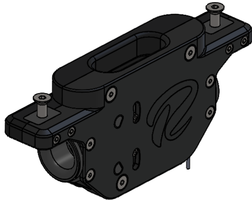
ISOMETRIC VIEW SCALE 1:3
