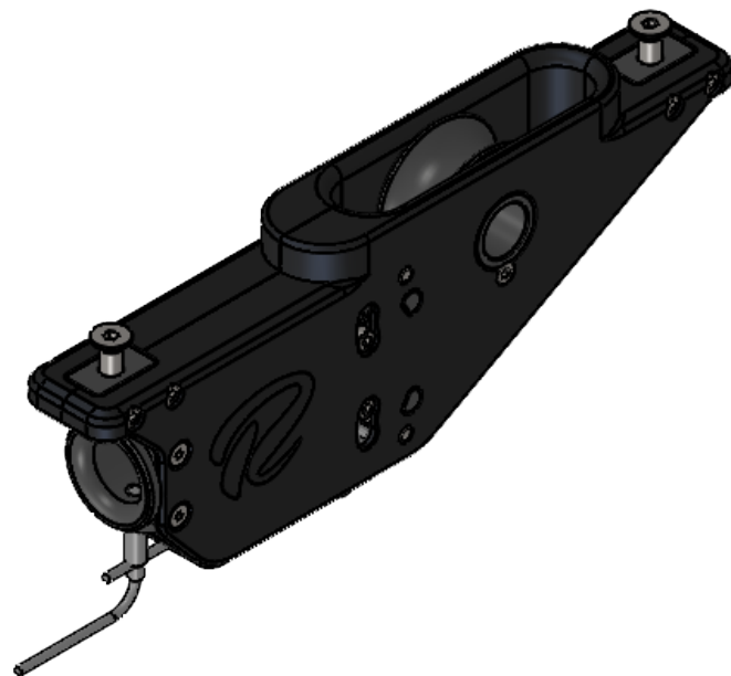
ISOMETRIC VIEW SCALE 1:3
