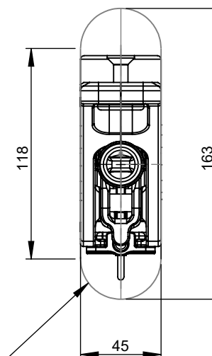
INSTALLATION CUT-OUT PROFILE
