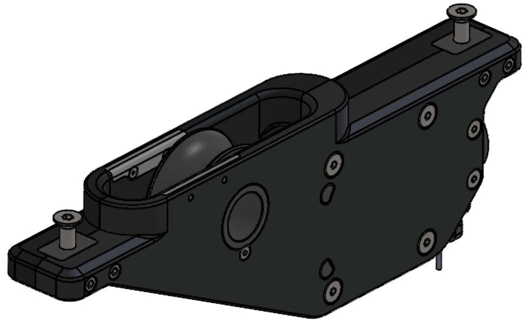
ISOMETRIC VIEW SCALE 1:3
