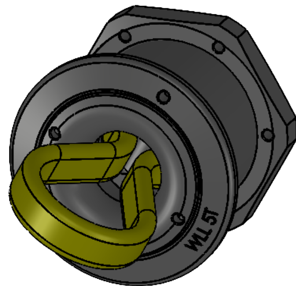
ISOMETRIC VIEW SCALE 1:1
