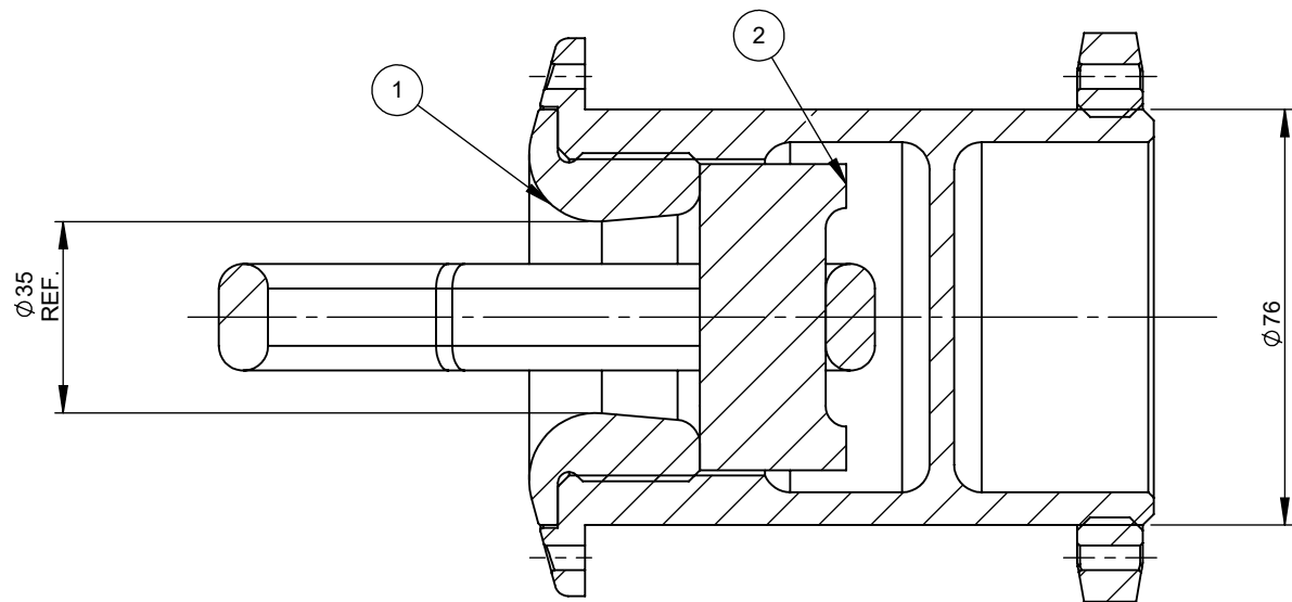
SECTION B-B
