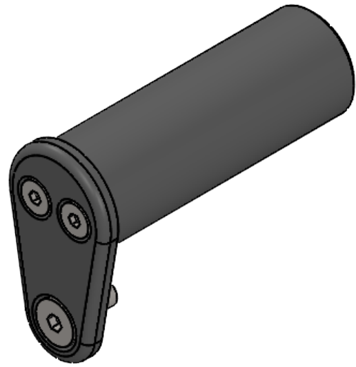
ISOMETRIC VIEW SCALE 2:3
