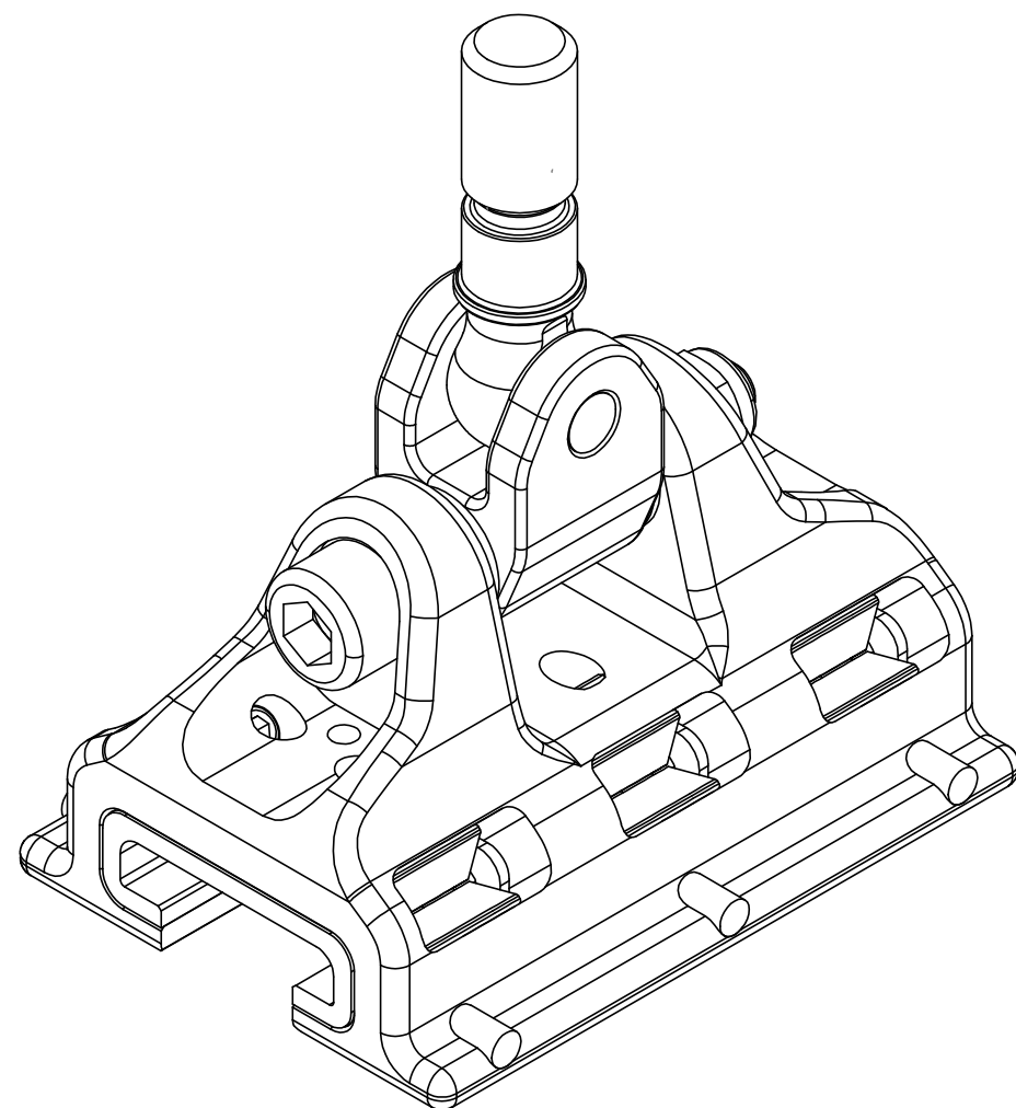
ISOMETRIC VIEW SCALE 1:1
