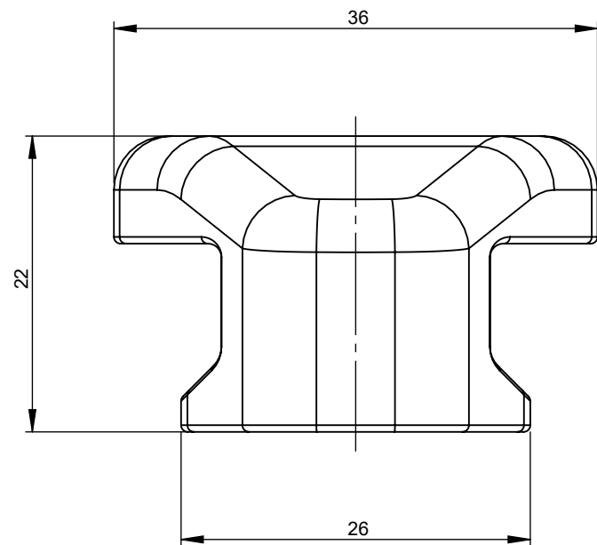
DETAIL X SCALE 2 : 1
