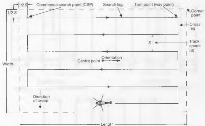
Parallel track search (PS)
