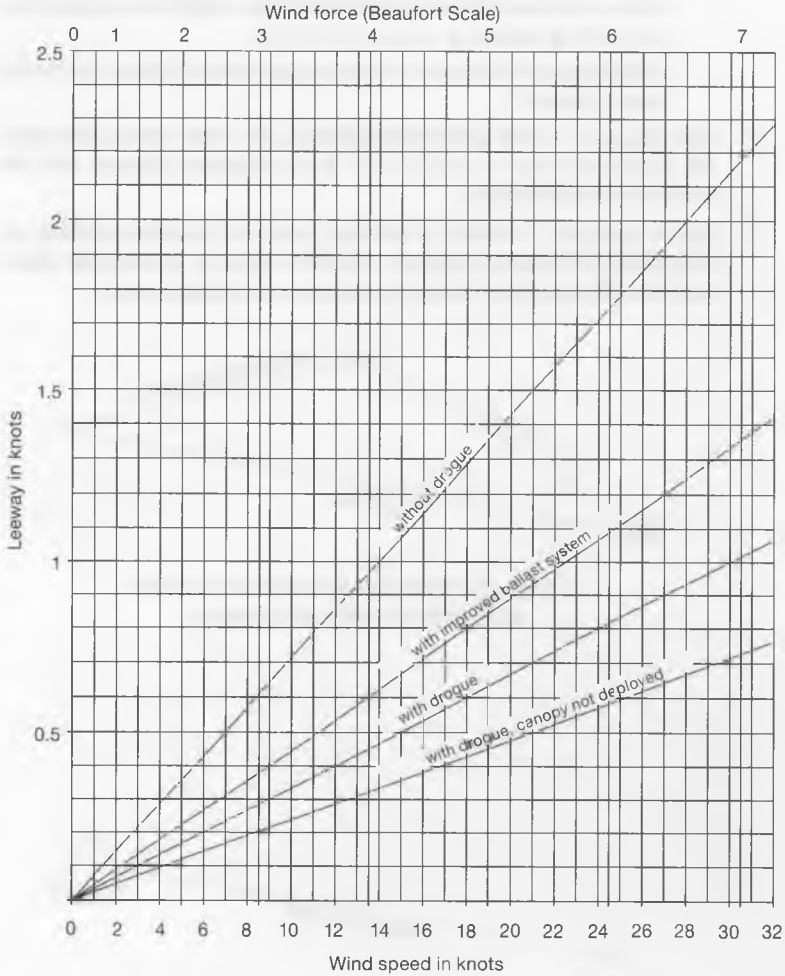
Liferaft leeway
