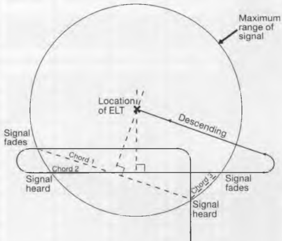
Map-assisted aural electronic search
