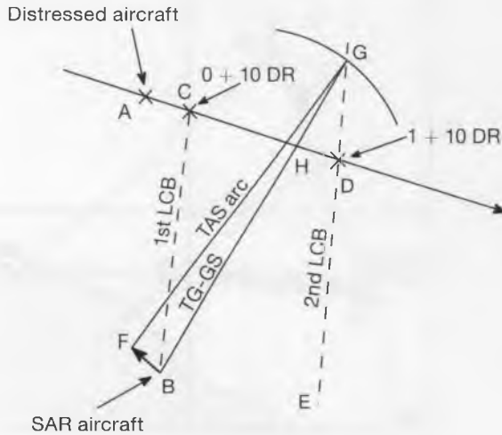
Offset or beam-on intercept: method 2
