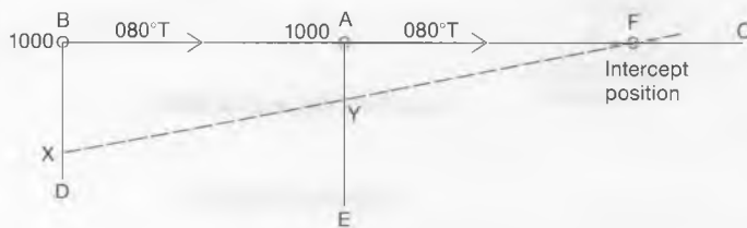
Overtaking method
