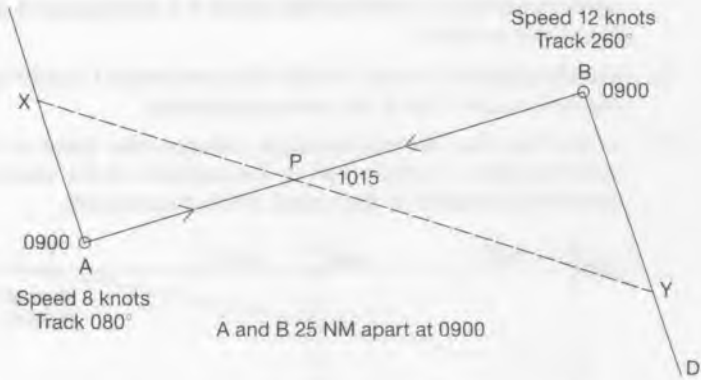
Head-on method
