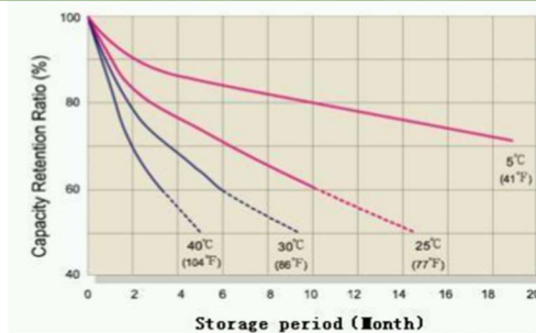
Capacity Retention Characteristic
