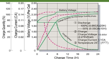
Battery Voltage and Charge Time for Standby Use
