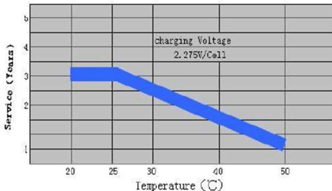
Tickle (or Float) Service Life
