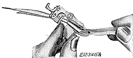
FIG. 42. INSERT FOLDED BINDING IN OUTSIDE SLOT
