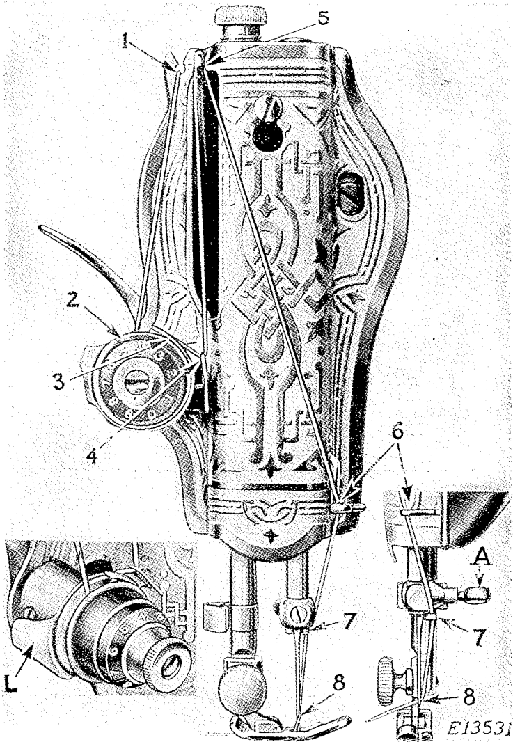
FIG. 12. UPPER THREADING
