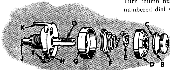
Fig. 25. Needle Thread Tension Disassembled
