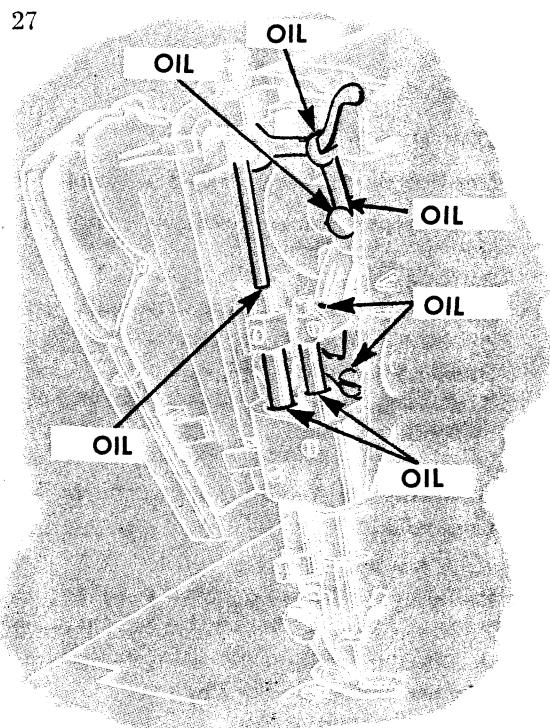
Fig. 31. Face Plate Opened Showing Oiling Points
