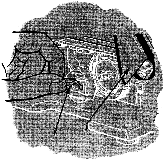
Fig. 8. Removing the Bobbin Case
