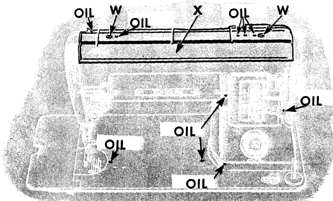
Fig. 29. Front View, Showing Oiling Points
