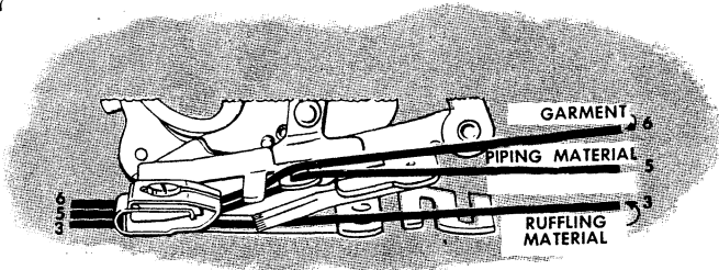
Fig. 68. Correct Positions for Materials
