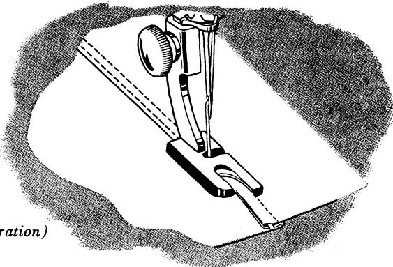
Fig. 40. Making a Felled Seam (First Operation)
