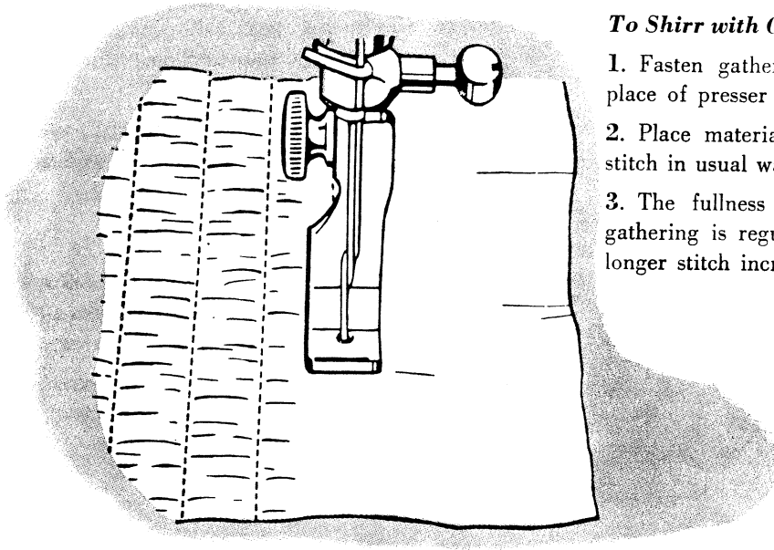
Fig. 60. Shirring with Gathering Foot
