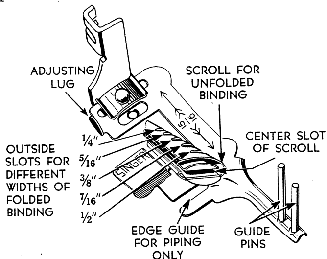
Fig. 45. Multi-Slotted Binder 160624
