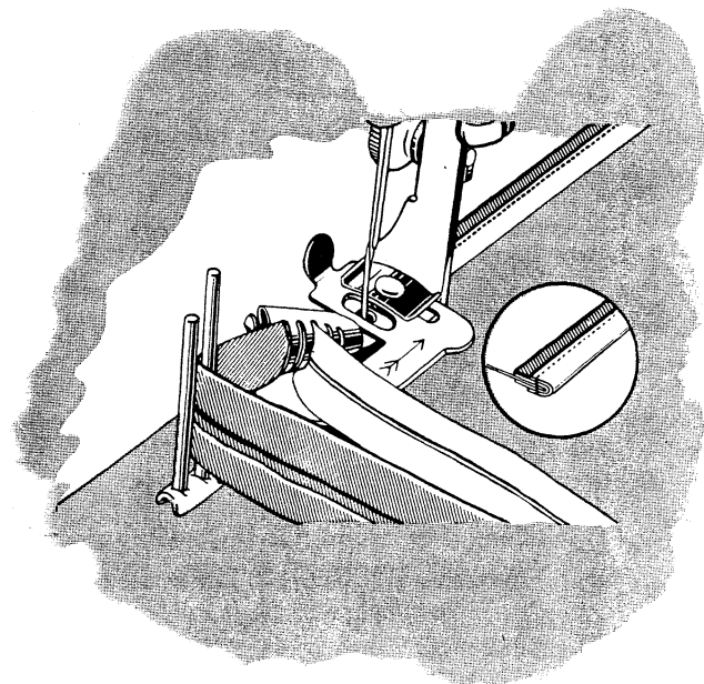
Fig. 49. Piping and Binding in One Operation
