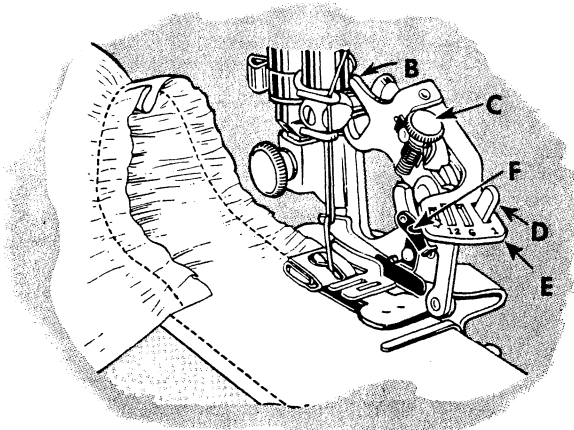
Fig. 62. Gathering with Ruffler
