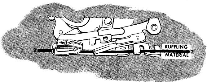
Fig. 70. Plaiting with Ruffler
