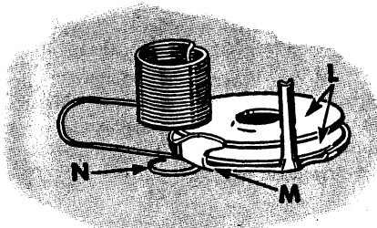
Fig. 26. Tension Disc Assembly
