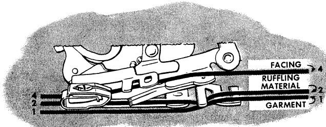
Fig. 66. Correct Positions for Materials
