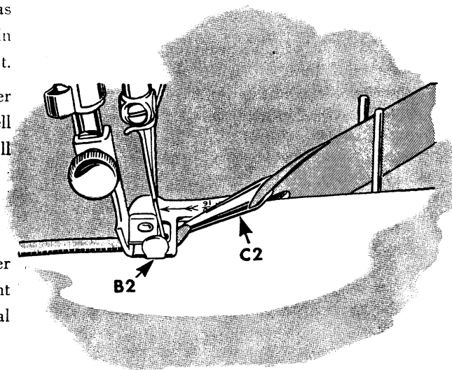
Fig. 47. Binding with Unfolded Bias Binding
