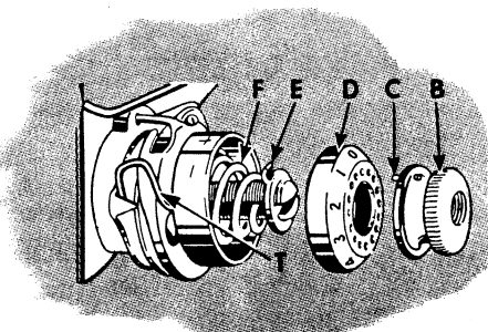
Fig. 27. Reassembling Needle Thread Tension
