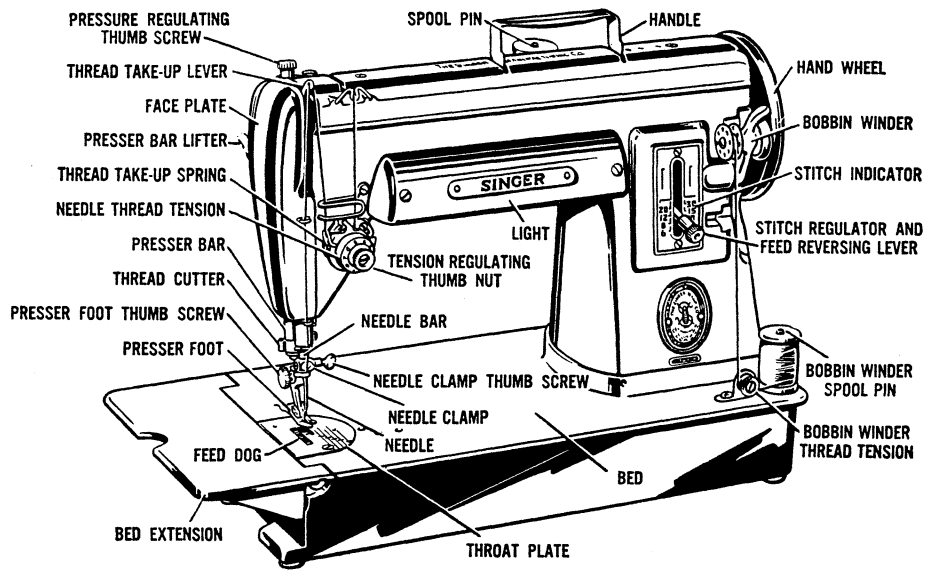
Fig. 34. Names of Principal Parts of Machine 301
