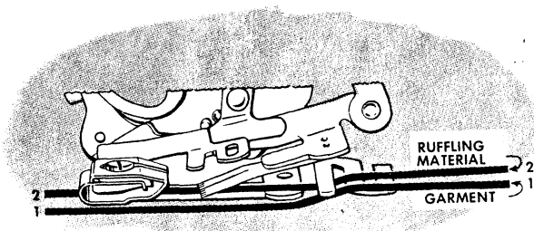
Fig. 64. Correct Positions for Materials
