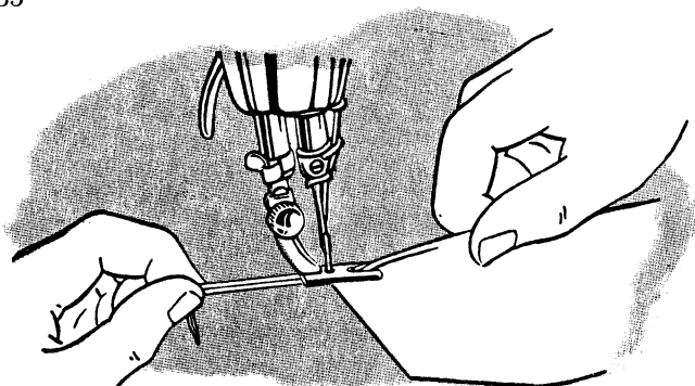
Fig. 36. Starting Hem at Very End of Material
