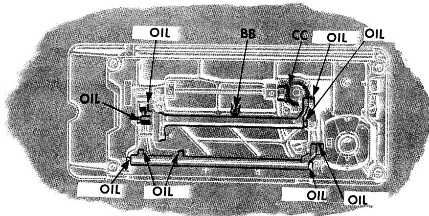
Fig. 33. Oiling Points in Base of Machine
