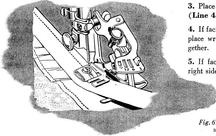
Fig. 66. Correct Positions for Materials
