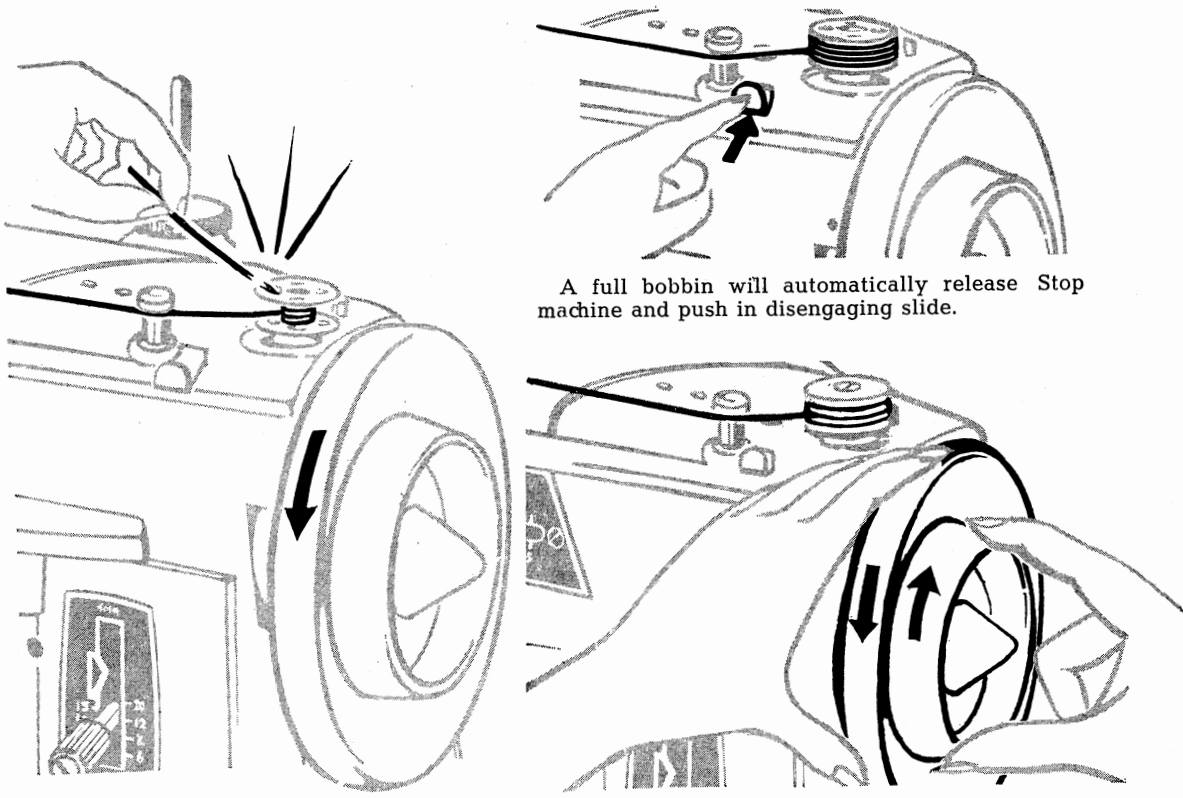
Tighten stop motion screw.
