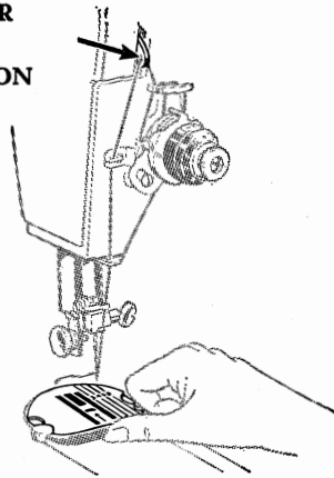
Throat plate raised (unlocked) for removal and replacement.
