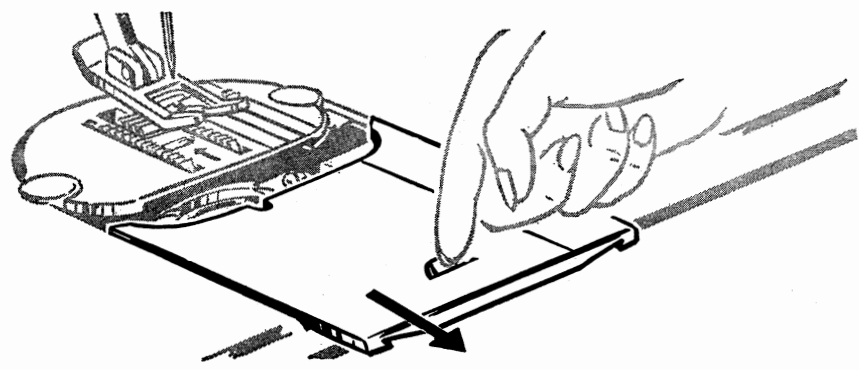
Open slide plate and remove bobbin.
