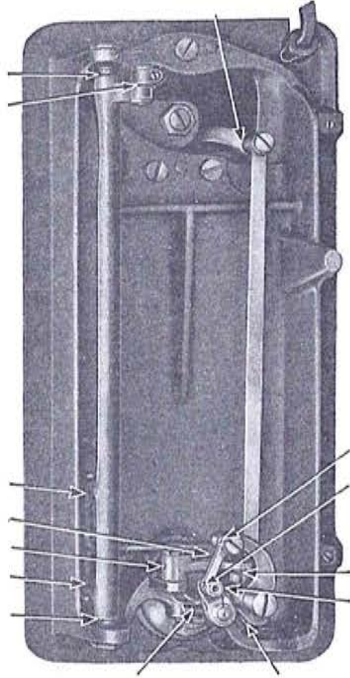
Fig. 28. Oiling Points in Base of Machine
