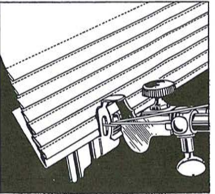
Fig. 58. Tucking with the Edge-Stitcher
