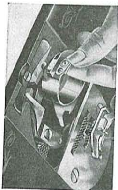
Fig. 32. Removing the Bobbin Case
