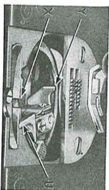
Fig. 33. Bobbin Case Position Bracket
