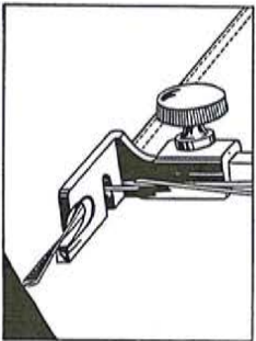
Fig. 39. Making a Hemmed Seam (Second Operation)
