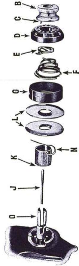
Fig. 21. Needle Thread Tension Disassembled
