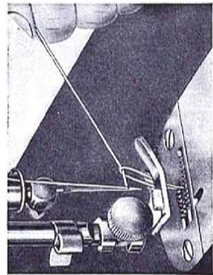
Fig. 12. Drawing Up the Under Thread
