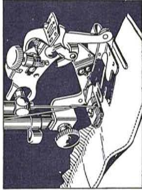
Fig. 65. Making a Ruffle and Attaching it in One Operation
