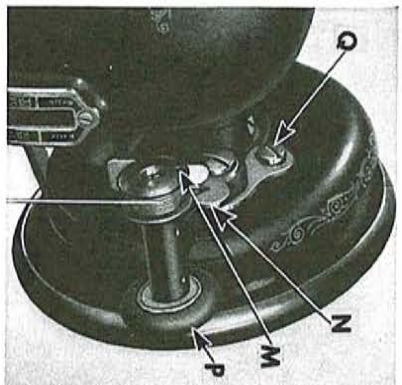
Fig. 5. Bobbin Winder Adjustment
