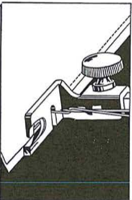
Fig. 40. Making a Filled Seam (First Operation)
