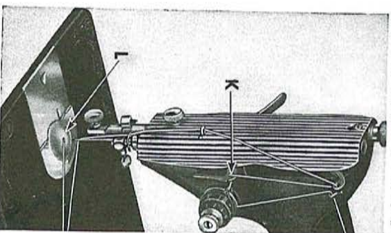
Fig. 75. Machine Threaded for Embroidery and Darning
