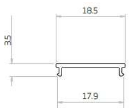
Tolerance(PC): \pm 0.3\text{mm}
