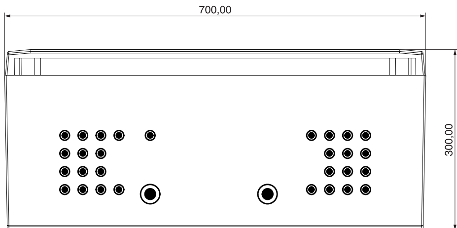
Figure 5-3 Housing dimensions - view from below
