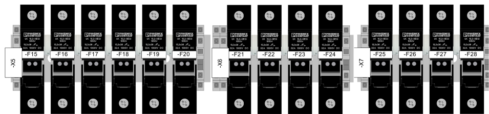
Figure 5-7 Fuse modular terminal blocks -F15 ... -F28
