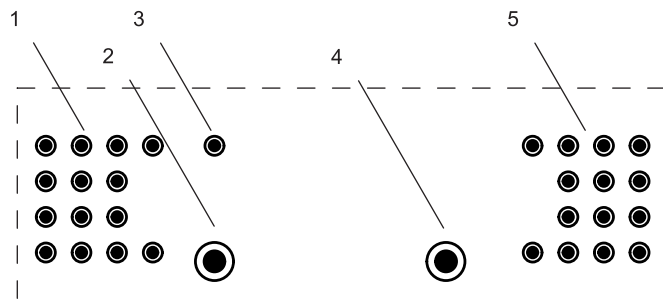
Figure 5-4 Cable feed-throughs on the underside of the housing (2 x M32, 29 x M16)
