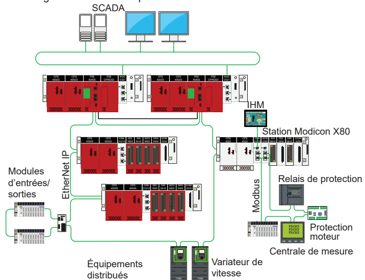
Topologie redondante Modicon M580 Safety
