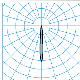
Faciella 20 RE2L/900-blue 1G1 TX046256 ■ CO - C180 DIN 5040: A80 UTE: 0,99 A CEN Flux Code: 98 99 100 100 99
