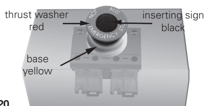
Mushroom-head pushbutton actuator "EMERGENCY STOP" GHG 410 1437R....
