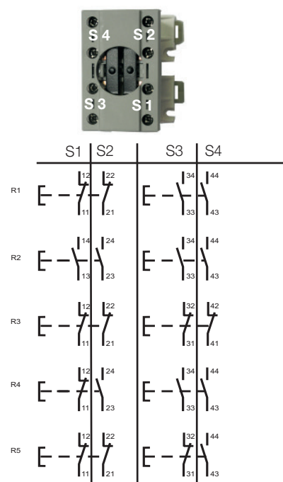
Contact arrangement
