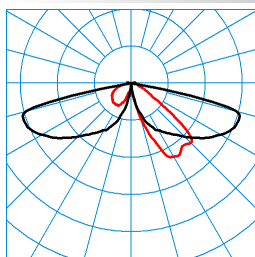
CS 19 100-AB2L-SLR1/5100-740 4G1S ET (CLO end value) TX300052 ■ C0 - C180 ■ C90 - C270 DIN 5040: A20 UTE: 1,00 l CEN Flux Code: 27 65 96 100 100 0 0 0 0
