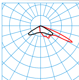
LnPlus 40-AM19L-SLR2/2200-727 2G1 ET (CLO end value) TX377022 DIN 5040: A30 UTE: 1,00 J CEN Flux Code: 28 76 99 100 100
