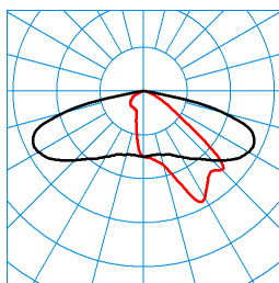
Jovie 50-AB2L-ML/1650-4200-740 4G1 ETDD (CLO initial value) TX271538 ■ C0 - C180 ■ C90 - C270 DIN 5040: A30 UTE: 1,00 G CEN Flux Code: 34 71 96 100 100
