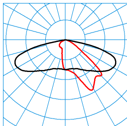
Jovie 50-AB2L-ML/1650-4200-740 4G1 ETDD (2400 lm) TX27351 ■ C0 - C180 ■ C90 - C270 DIN 5040: A30 UTE: 1,00 G CEN Flux Code: 34 71 96 100 100
