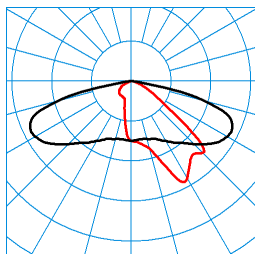
Jovie 50-AB2L-ML/1650-4200-740 4G1 ETDD (4200 lm) TX27352 ■ C0 - C180 ■ C90 - C270 DIN 5040: A30 UTE: 1,00 G CEN Flux Code: 34 71 96 100 100
