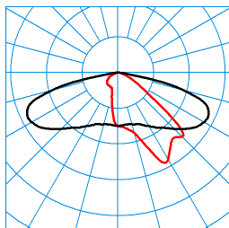
Jovie 50-AB2L-ML/1650-4200-740 4G1 ETDD (CLO end value) TX271486 ■ C0 - C180 ■ C90 - C270 DIN 5040: A30 UTE: 1,00 G CEN Flux Code: 34 71 96 100 100
