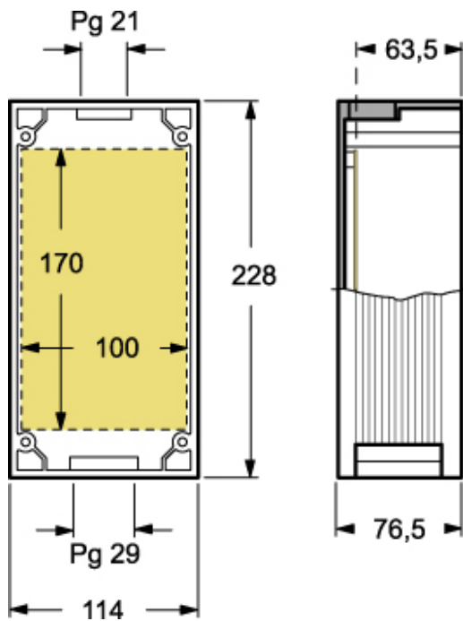
Catalogue drawings
