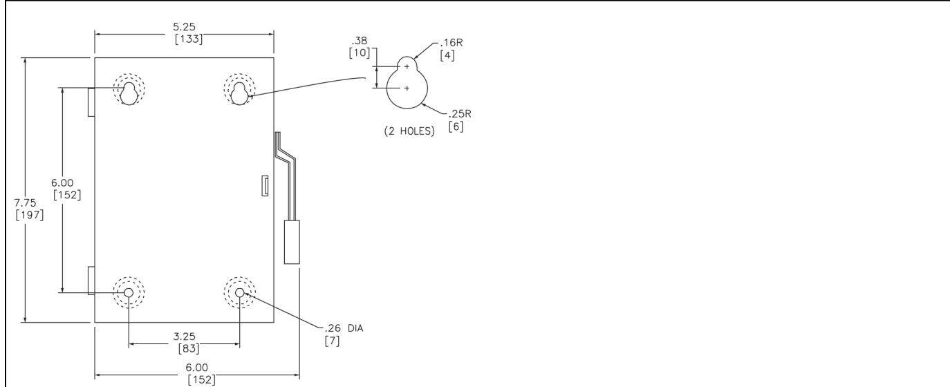
Type 1 – 30 A
