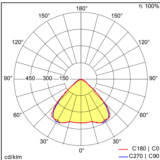
D45564_CR2PL_M17k-840_PM_VWB_LDO.idt
