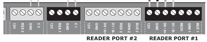
ENTRANCE READER
