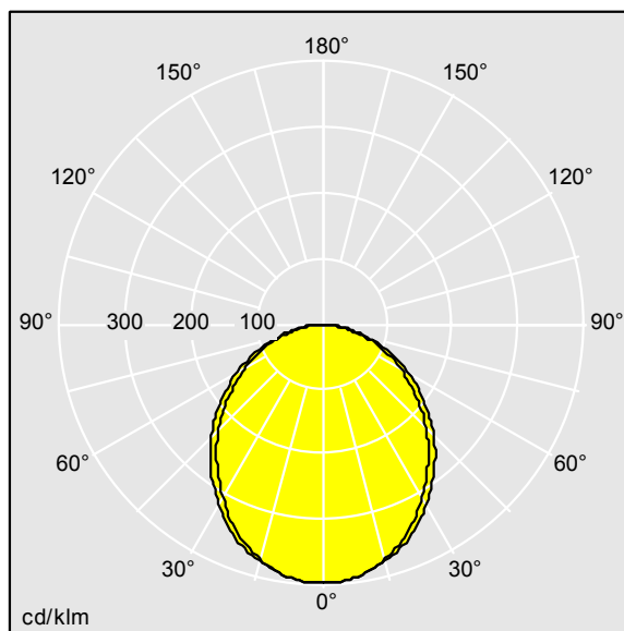
D44260AA_EQL_840_HF_L1250_PM_SR_.ldt
