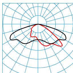
Jovie 70-AB7L-ML/75-150-740 12G1 ETDD (CLO initial value) TX271537 ■ C0 - C180 ■ C90 - C270 DIN 5040: A30 UTE: 1,00 G CEN Flux Code: 34 72 96 100 100
