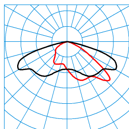
Jovie 70-AB7L-ML/75-150-740 12G1 ETDD (CLO end value) TX271563 ■ C0 - C180 ■ C90 - C270 DIN 5040: A30 UTE: 1,00 G CEN Flux Code: 34 72 96 100 100
