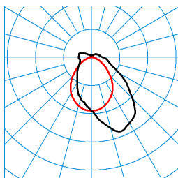
TugraHE 18 PAW 65-100/16ML-830 ET PC 23 (STAG15) TX425094
