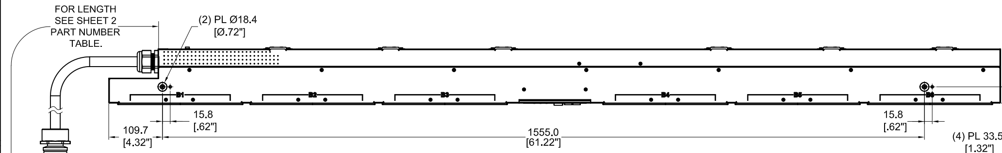
RIGHT VIEW
