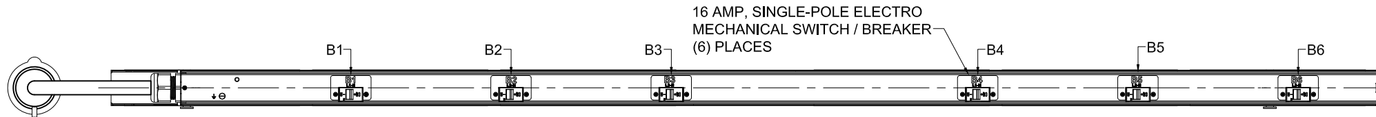
REAR VIEW
