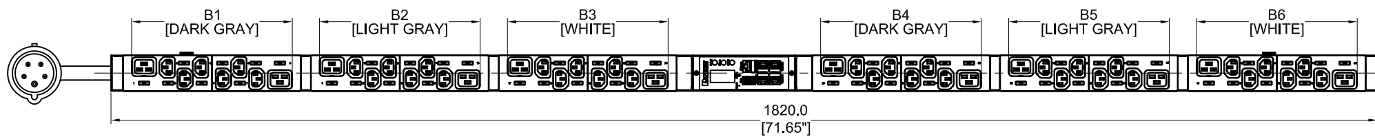
FRONT VIEW
