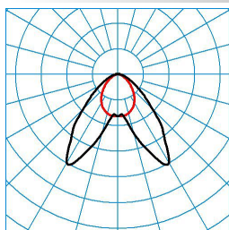
ELINE FL LDAW120 865 L225 1 20
