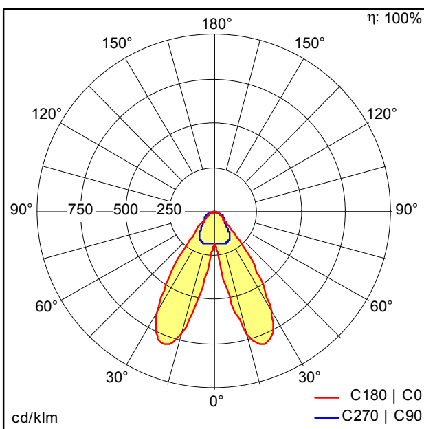
D43656AA_TECTON_C_LED7400-830_L2000_SB_LDE_BK.Idt
