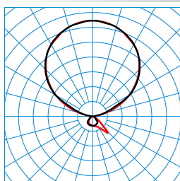
Luceos Act S G2 PAW-IL 150 ETDI 05+LLWP (ActDWW) TX299620 ■ C0 - C180 ■ C90 - C270 DIN 5040: E43 UTE: 0.10 D + 0.90 T DLOR: 10 % ULOR: 90 % CEN Flux Code: 52 86 97 10 100 49 82 98 90
