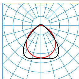
ELINE HE PW60 840 L150 1 50
