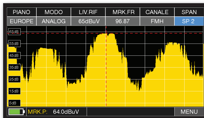
Spectre FM SPAN 2 MHz
