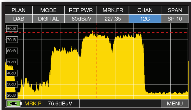
Spectre DAB SPAN 10 MHz.
