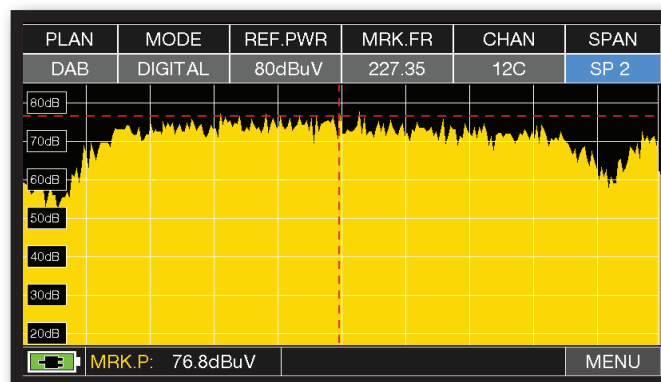
Spectre "DAB" SPAN 2 MHz.
