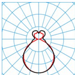
ELINE HE PWW40-120 ML 830 L150 4 20 ■ C0 - C180
