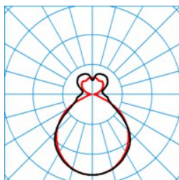
ELINE HE PWW40-120 ML 830 L150 2 20 ■ C0 - C180
