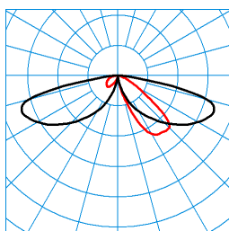
LTX LT-AB2L-LRA/15/18/26-730 4G1 (2600 lm) TX084096 ■ C0 - C180 ■ C90 - C270 DIN 5040: A20 UTE: 1,00 l CEN Flux Code: 23 60 91 100 100 0 0 0 0
