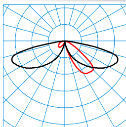
LTX LT-AB2L-LRA/15/18/26-730 4G1 (1500 lm) TX084094 ■ C0 - C180 ■ C90 - C270 DIN 5040: A20 UTE: 1,00 l CEN Flux Code: 23 60 91 100 100 0 0 0 0
