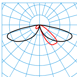
LTX LT-AB2L-LRA/15/18/26-730 4G1 (1800 lm) TX084095 ■ C0 - C180 ■ C90 - C270 DIN 5040: A20 UTE: 1,00 l CEN Flux Code: 23 60 91 100 100 0 0 0 0
