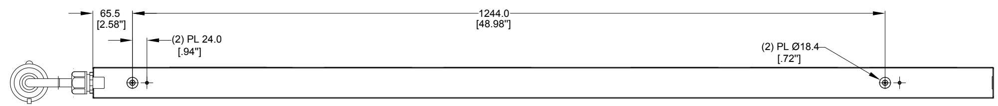
REAR VIEW
