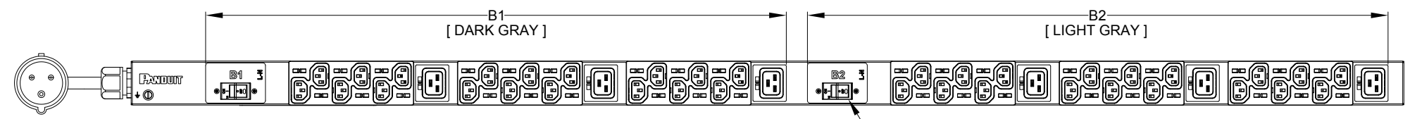
FRONT VIEW
