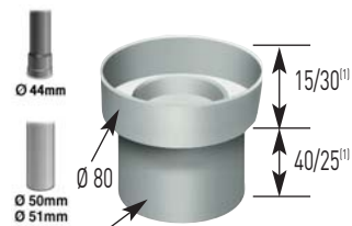
Raccord
