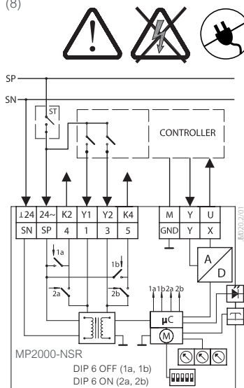
MP2000-NSR operating as modulating version (8)
