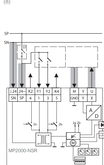
MP2000-NSR operating as floating version (8)
