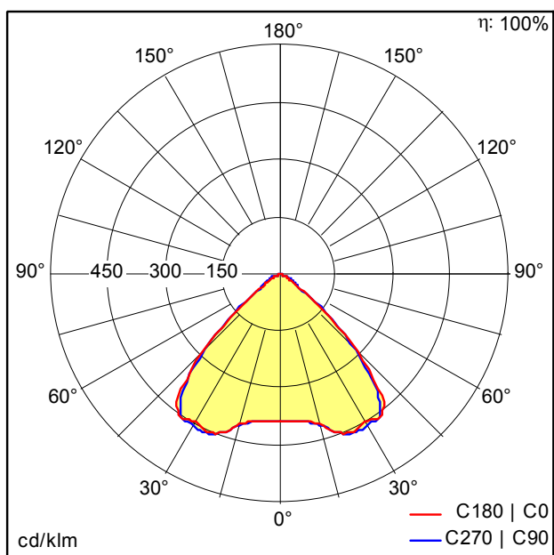
D45565_CR2_M21k-840_PC_VWB_LDO.idt
