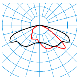
Jovie 70-AB7L-LR/24000-730 24G1 ET (CLO initial value) TX301539 ■ C0 - C180 ■ C90 - C270 DIN 5040: A30 UTE: 1,00 G CEN Flux Code: 35 73 97 100 100
