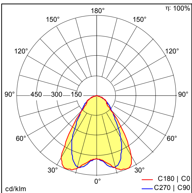
D44421AA_TEC_LED5200-840_L1000_WB_LDE_WH_IP.ltd
