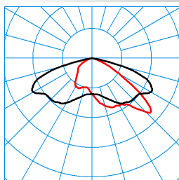
LnPlus 60-AB7L/26000-740 24G1 ETDD (CLO end value) TX390089 ■ C0 - C180 ■ C90 - C270 DIN 5040: A30 UTE: 1,00 G CEN Flux Code: 35 73 98 100 100
