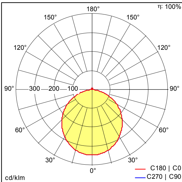
D36853AA_ONDA2_P_D590_LED5800-830.ltd
