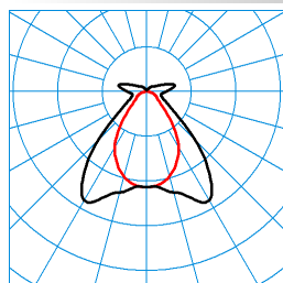
TugraHE Act 12 PW19 40 ETDD8 01 (ACTDWW) TX303626 ■ C0 - C180 ■ C90 - C270 DIN 5040: B41 UTE: 0,81 D + 0,19 T CEN Flux Code: 60 85 94 81 100 9 28 64 19
