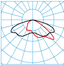
LnPlus 40-AB7L/8200-727 8G1 ETDD (CLO end value) TX377743 ■ C0 - C180 ■ C90 - C270 DIN 5040: A30 UTE: 1,00 G CEN Flux Code: 35 73 98 100 100
