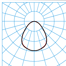
7651IP MironaF B 270-840ET L225 01 (LEO1) TX306221 ■ C0 - C180 ■ C90 - C270 UGR I = 29,0 UGR q = 28,2 DIN 5040: A50 UTE: 1,00 D CEN Flux Code: 58 87 98 100 100
