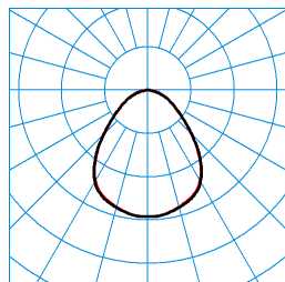
7651IP MironaF B 270-840ET L225 01 (LEO3) TX306218 ■ C0 - C180 ■ C90 - C270 UGR I = 29,0 UGR q = 28,2 DIN 5040: A50 UTE: 1,00 D CEN Flux Code: 58 87 98 100 100
