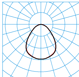
7651IP MironaF B 270-840ET L225 01 (LEO2) TX306205 ■ C0 - C180 ■ C90 - C270 UGR I = 29,0 UGR q = 28,2 DIN 5040: A50 UTE: 1,00 D CEN Flux Code: 58 87 98 100 100
